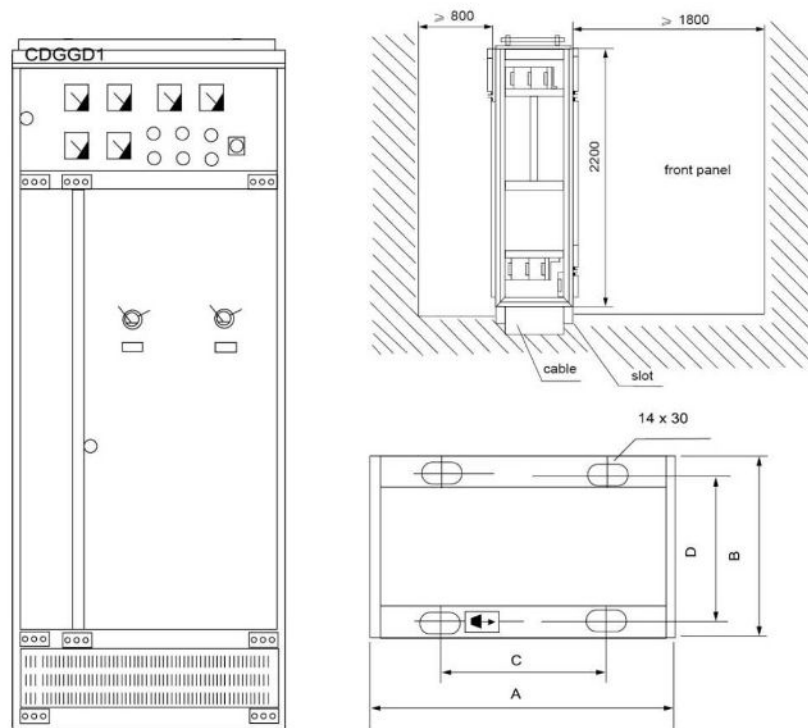
Figure 2. Mounting dimensions of CDGGD1 AC low voltage distribution switchgear
